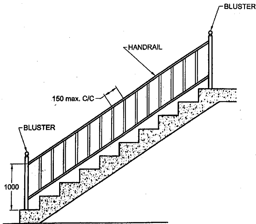
FIG. 1 TYPICAL DETAIL FOR HANDRAIL/BLUSTERS OF A STAIRCASE
