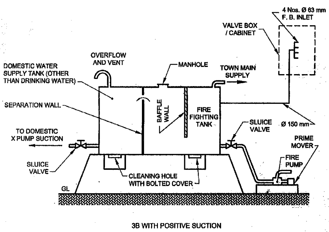
FIG. 6 TYPICAL ARRANGEMENT FOR PROVIDING COMBIND FIRE FIGHTING AND DOMESTIC WATER STORAGE TANK
